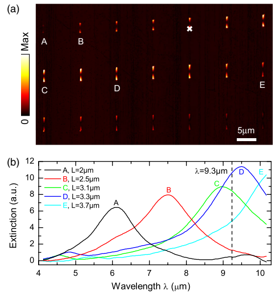
FIG. 3 (color online). Experimental near- and far-field study of linear infrared dipole antennas. (a) s -SNOM image of the nano-antennas at \lambda = 9.3 \mu\text{m} . From the top to the bottom and from the left to the right, the antenna length increases from L = 2 \mu\text{m} to L = 4.4 \mu\text{m} . The cross indicates the position where the near-field intensities displayed in Fig. 4 have been measured. (b) Far-field extinction spectra of the antennas marked in Fig. 3(a) by the letters A-E. The vertical dashed line indicates the wavelength \lambda = 9.3 \mu\text{m} , where the extinction values displayed in Fig. 4 have been extracted.
