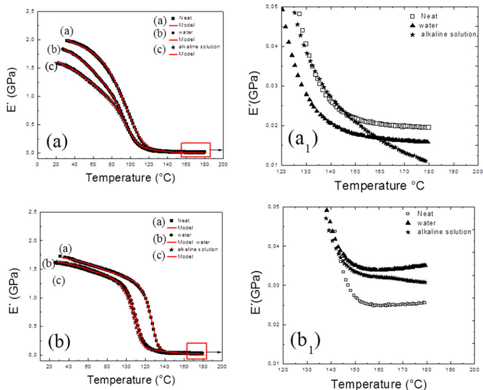
FIGURE 12. Modeling of storage modulus at the rubbery state after immersion in water and in the alkaline solution at 50°C. (a) Unsaturated polyester resin and (b) epoxy resin. (a 1 ) Closer view of the unsaturated polyester resin in the rubbery state. (b 1 ) Closer view of the epoxy resin in the rubbery state.
