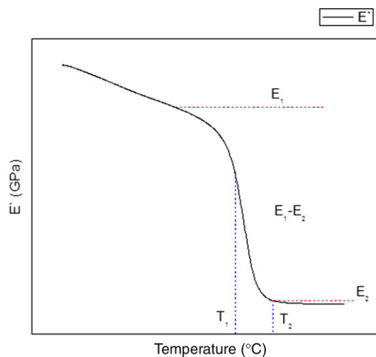
FIGURE 11. Reference values for model calculations.
