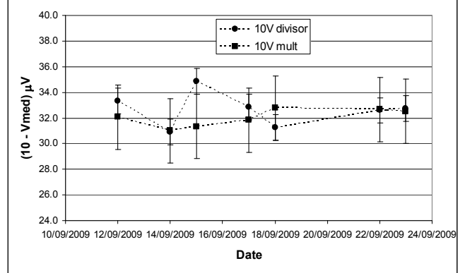
Figure 4. Comparison of 10 V measurements using both methods.
