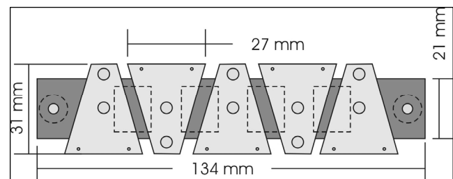
Figure 2. Tetrahedral cooper junctions
