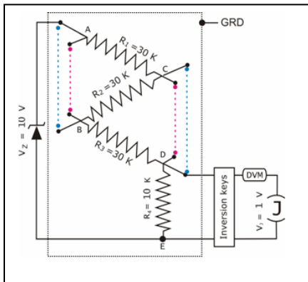
Figure 3. Diagram of connections to measure 10 V zener output with JVS using the divider. Dotted lines A,B and C,D terminals correspond to short circuits used to perform divider ratio calibration.
