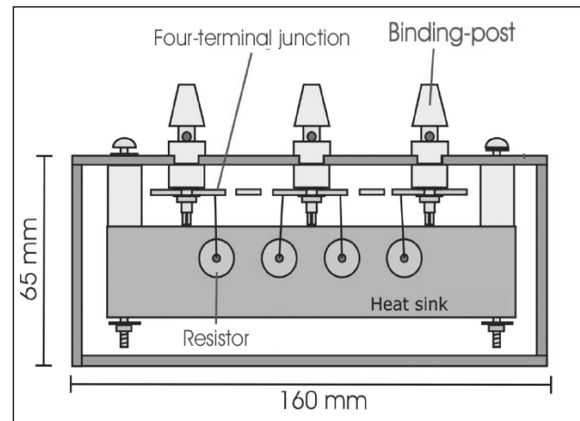
Figure 1. Lateral view of the divider
